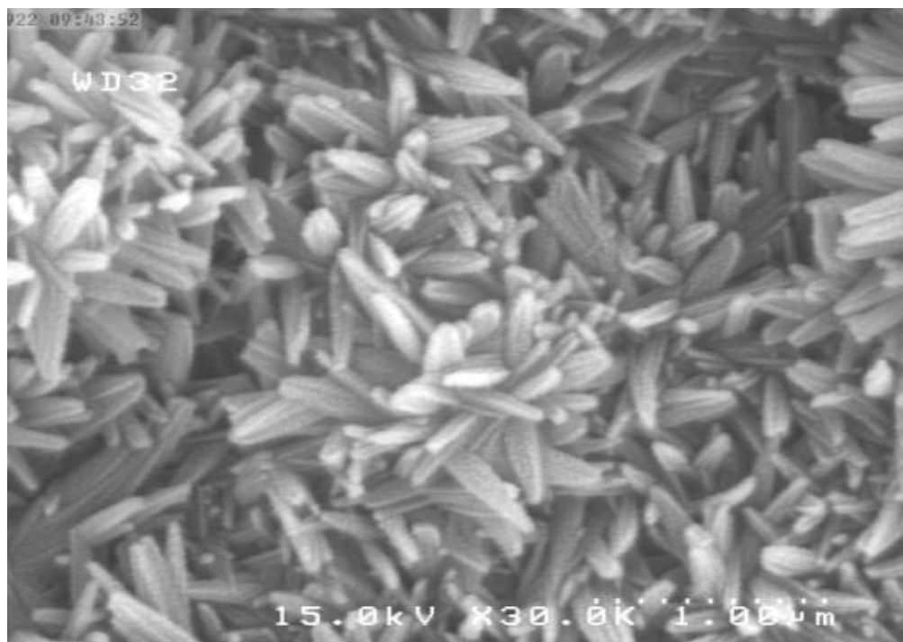
Scheme 1. The SEM image of \text{Ti}_2\text{O}_3 nanoparticles produced by calcination of [\text{Ti}(\text{PsucH})]_n .
