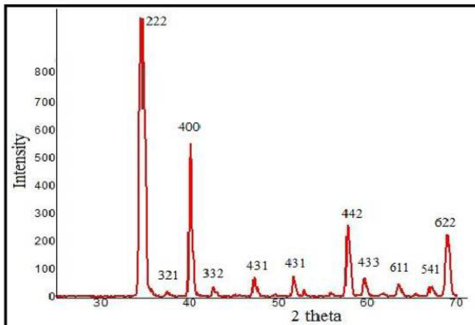
Fig 1. The XRD pattern of \text{Ti}_2\text{O}_3 produced by calcinations of [\text{Ti}(\text{PsucH})]_n .
