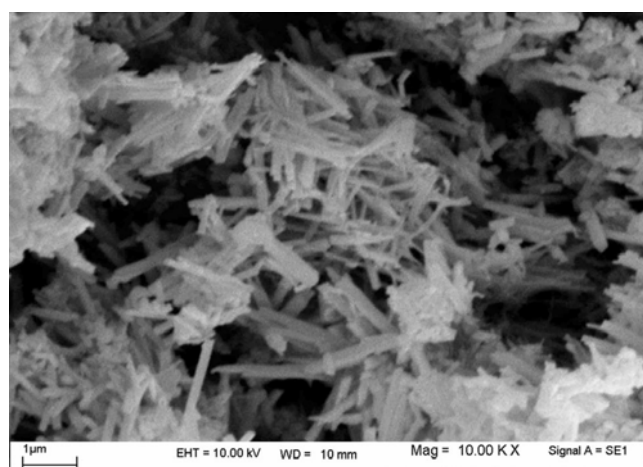
Fig. 2. SEM images of PbWO 4 nanostructures.
