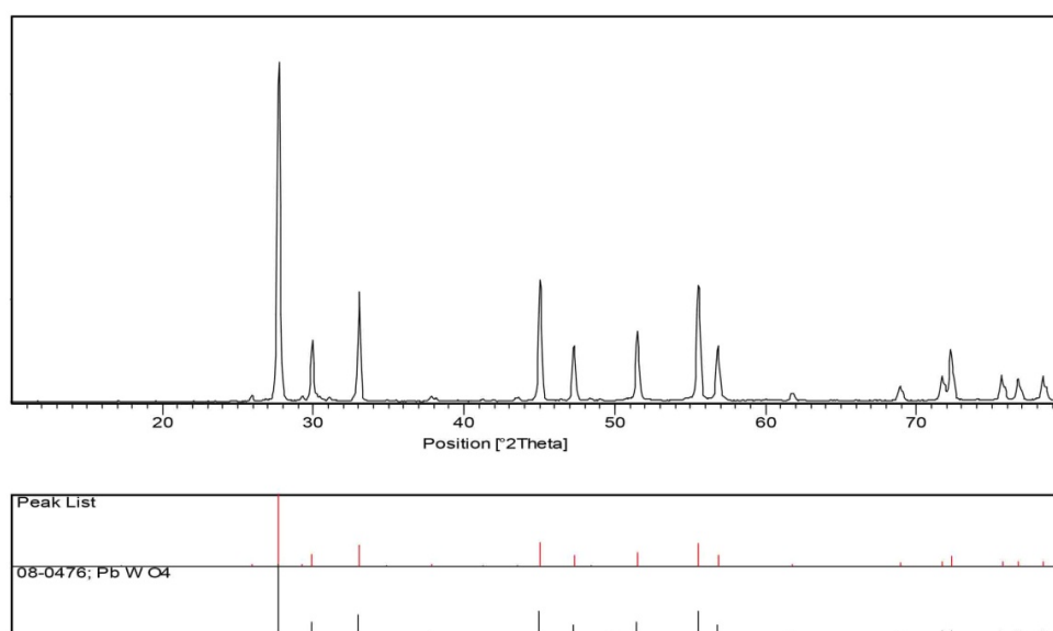
Fig. 1. XRD pattern of PbWO 4 nanostructures.
