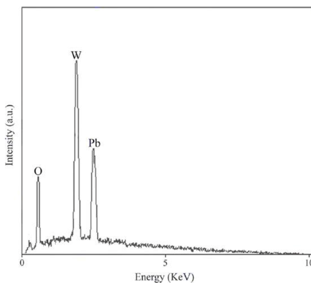
Fig.4. EDS spectrum of PbWO 4 nanostructures.
