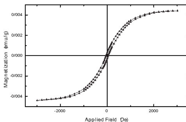
Fig 3. VSM curve of PbWO 4 nanostructures.
