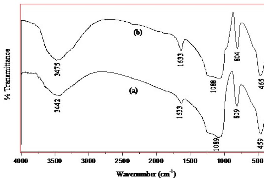
Fig. 3. FT-IR spectrum of (a) MCM-22 zeolite (b) Fe-MCM-22 zeolite.
