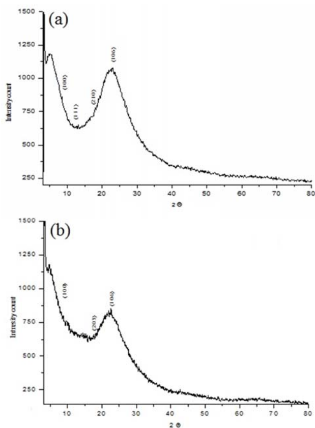
Fig. 1. Powder XRD pattern of (a) MCM-22 Zeolite (b) Fe-MCM-22 Zeolite.
