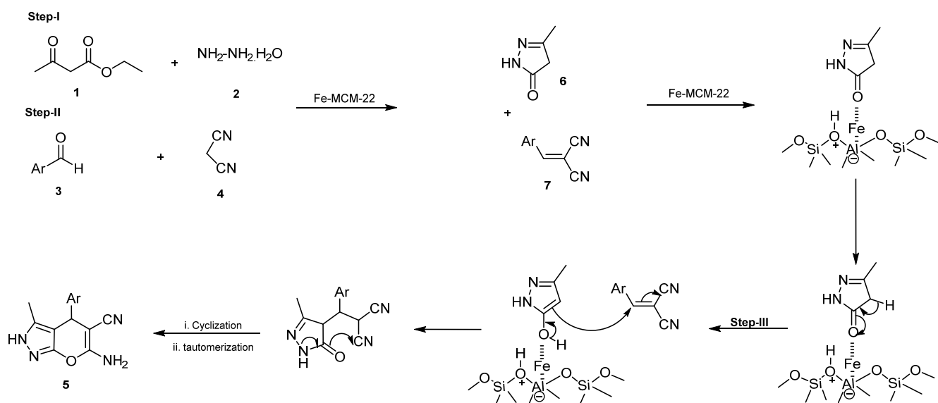
Scheme 2. Plausible Mechanism for the formation of dihydropyrano [2, 3-c] pyrazoles.
