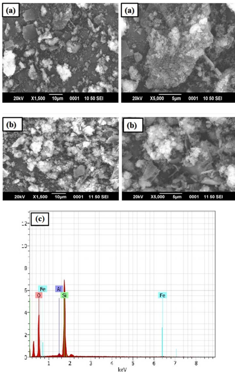
Fig. 2. (a) SEM-images of MCM-22 zeolite (b) SEM-images of Fe-MCM-22 zeolite and (c) EDS Spectrum of Fe-MCM-22 zeolite.
