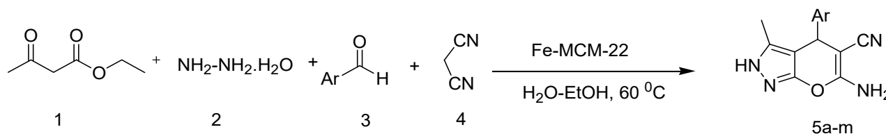
Scheme1. Synthesis of dihydropyrano [2, 3-c] pyrazole derivatives.
