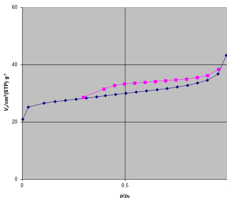
Fig. 4. N 2 adsorption-desorption isotherms of HMCM-22.
