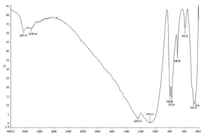
Fig. 2. FT-IR spectrum of HMCM-22
