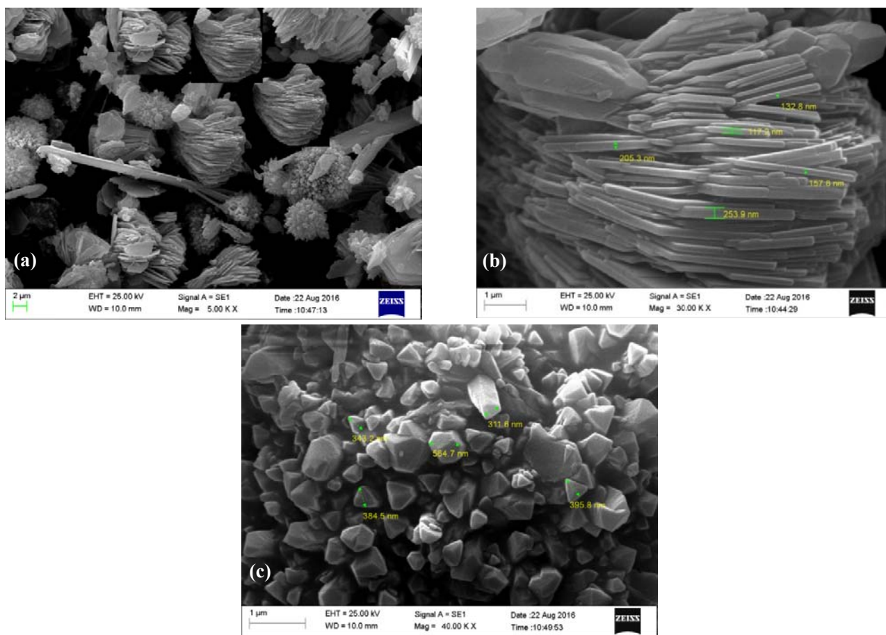
Fig. 1. SEM images of HMCM-22. Wide view (a), lamellar structures (b), and aggregated spherical particles (c).
