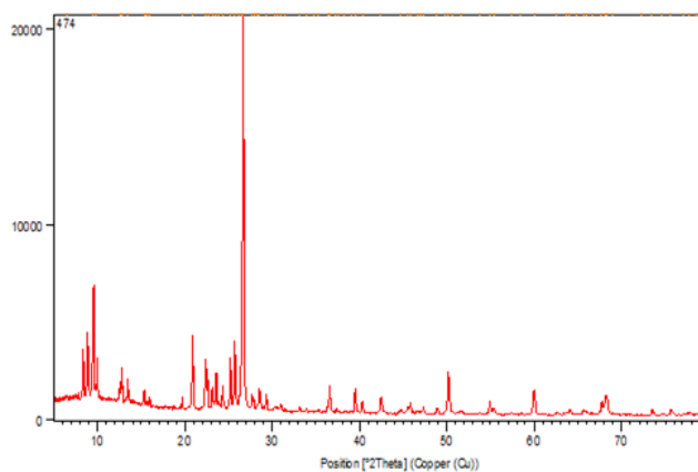
Fig. 3. X-ray diffraction pattern of HMCM-22
