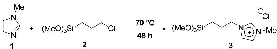
Scheme 1. Synthesis of N -methyl- N' -propyl trimethoxysilylimidazolium chloride.
