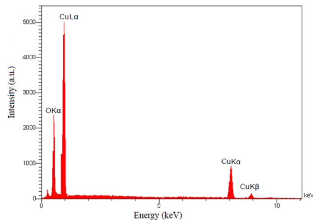
Fig. 4. EDS spectrum of CuO NPs.
