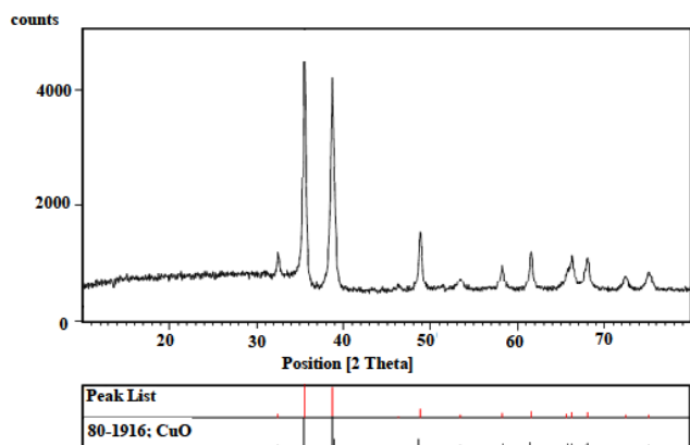
Fig. 2. The XRD pattern of CuO NPs.
