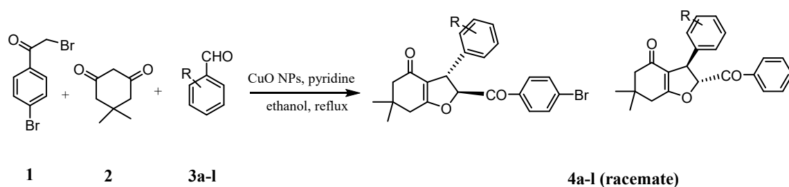
Scheme 1. Synthesis of dihydrofurans using biosynthesized CuO nanoparticles
