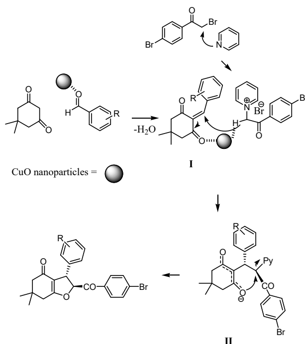
Scheme 3. Possible mechanism for the synthesis of trans -2,3-dihydrofuran using CuO NPs.
