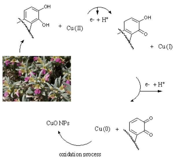
Scheme 2. Reducing ability of antioxidant phenolics of Ajuga chamaecistus Subsp. Scoparia extract to produce nanoparticles.
