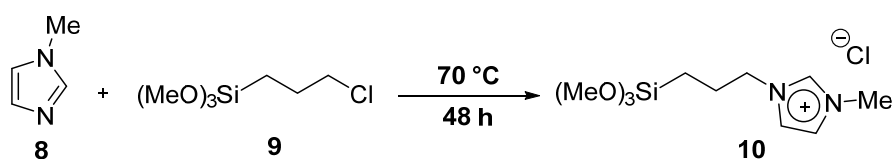
Scheme 3. Synthesis of N -methyl- N' -propyl trimethoxysilylimidazolium chloride
