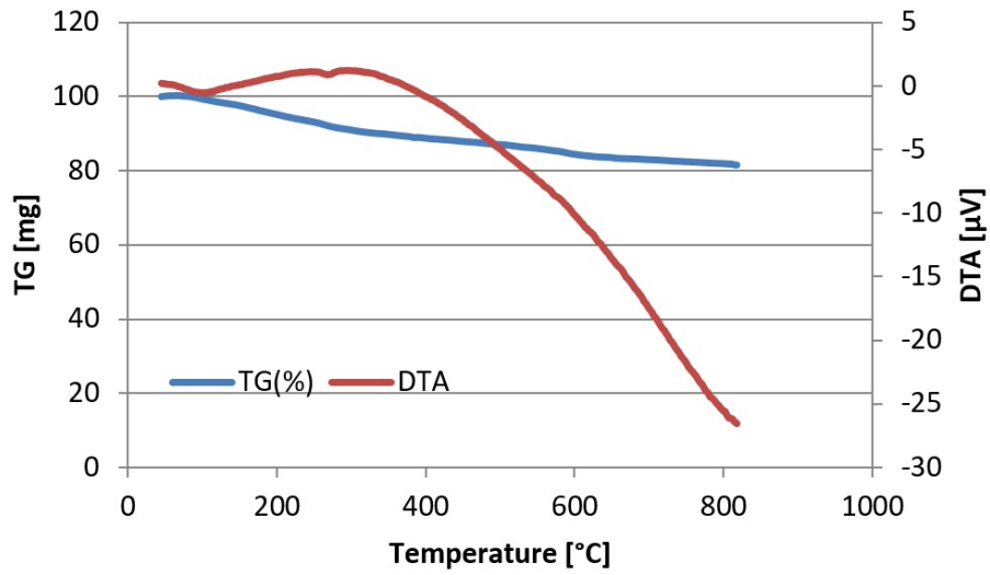
Fig. 4. Thermal gravimetric analysis (TG-DTG) pattern of egg white nano-ovalbumin.
