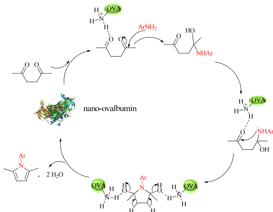
Scheme 2. Plausible mechanism for egg white ovalbumin catalyzed Paal-Knorr reaction.
