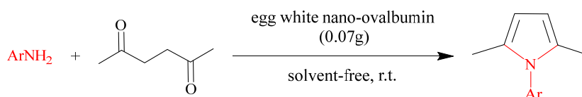
Scheme 1. Egg white nano-ovalbumin-catalyzed Paal-Knorr reaction.
