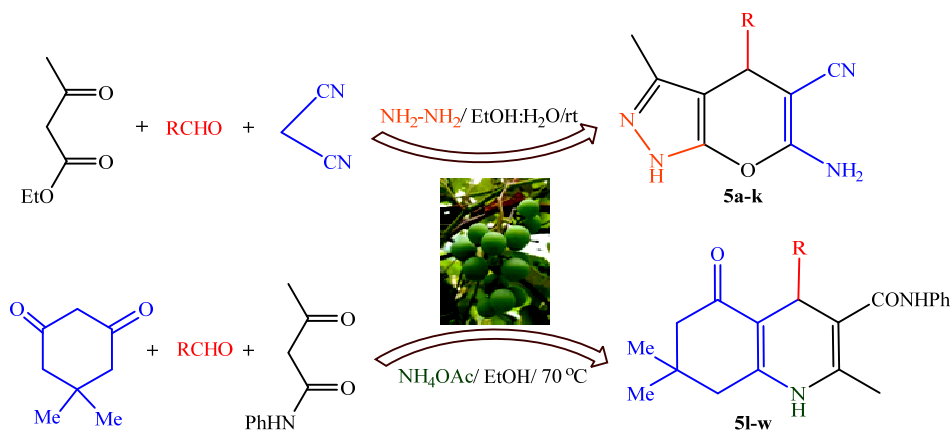
Scheme 1. Synthesis of pyranopyrazoles and hexahydroquinoline-3-carboxamides catalyzed by verjuice.
